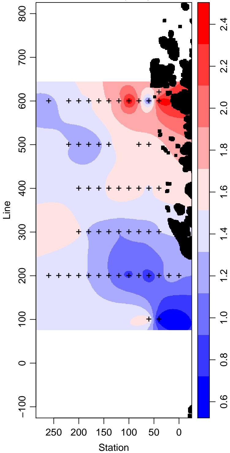
LMG07-01_15_Phosphate \mu\text{ mol L}^{-1}
