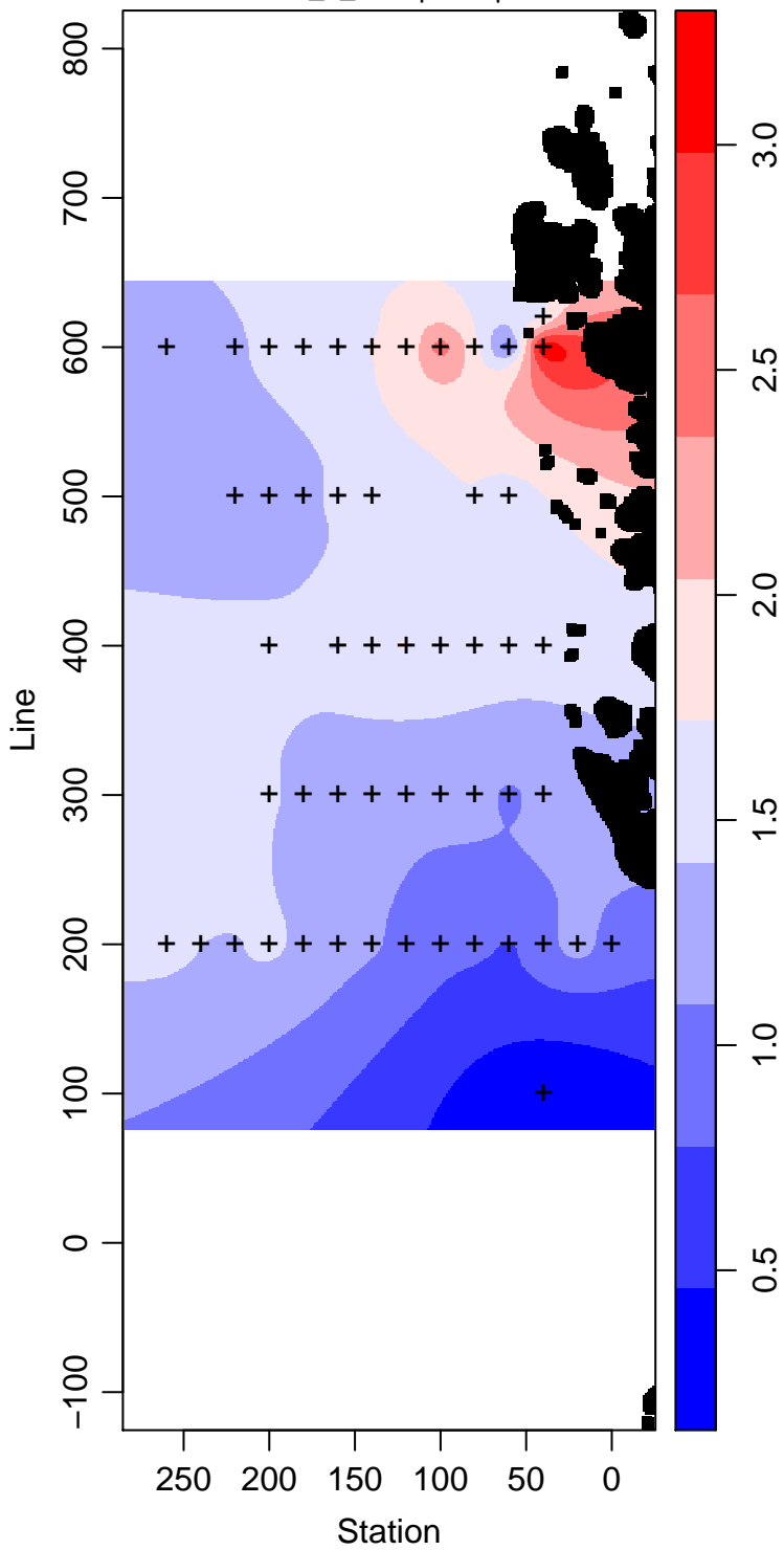
LMG07-01_1_Phosphate \mu\text{ mol L}^{-1}
