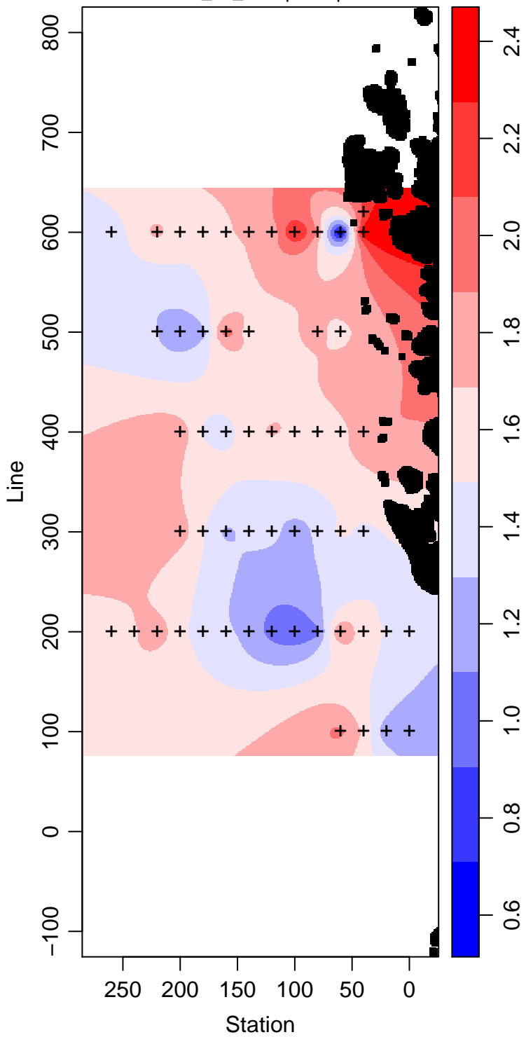
LMG07-01_30_Phosphate \mu\text{ mol L}^{-1}
