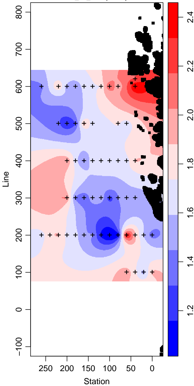
LMG07-01_35_Phosphate \mu\text{ mol L}^{-1}
