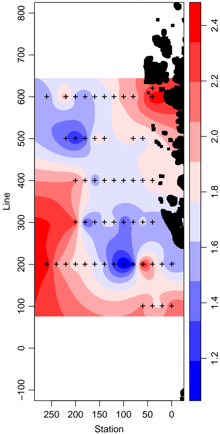
LMG07-01_40_Phosphate \mu\text{ mol L}^{-1}
