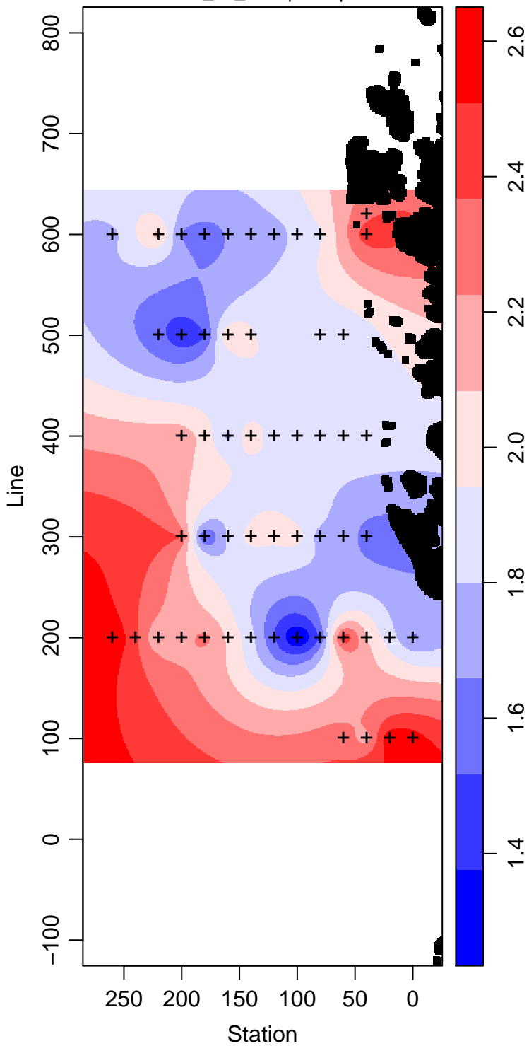
LMG07-01_50_Phosphate \mu\text{ mol L}^{-1}
