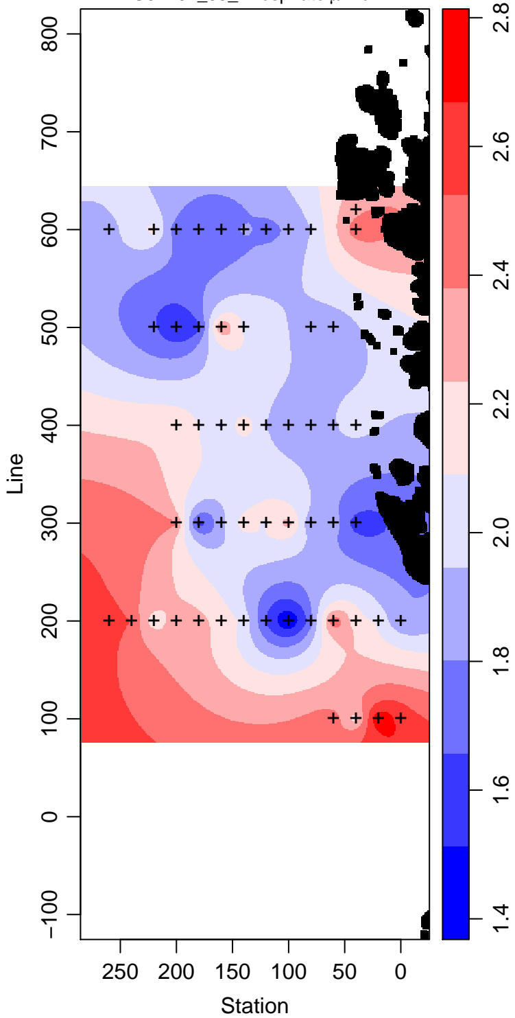
LMG07-01_55_Phosphate \mu\text{ mol L}^{-1}
