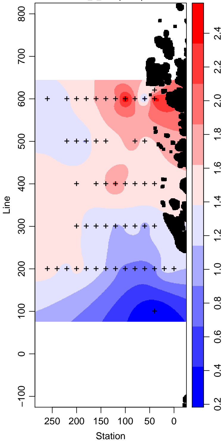
LMG07-01_5_Phosphate \mu\text{ mol L}^{-1}
