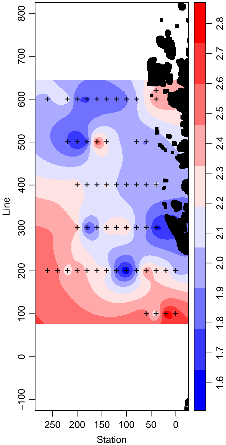
LMG07-01_60_Phosphate \mu\text{ mol L}^{-1}
