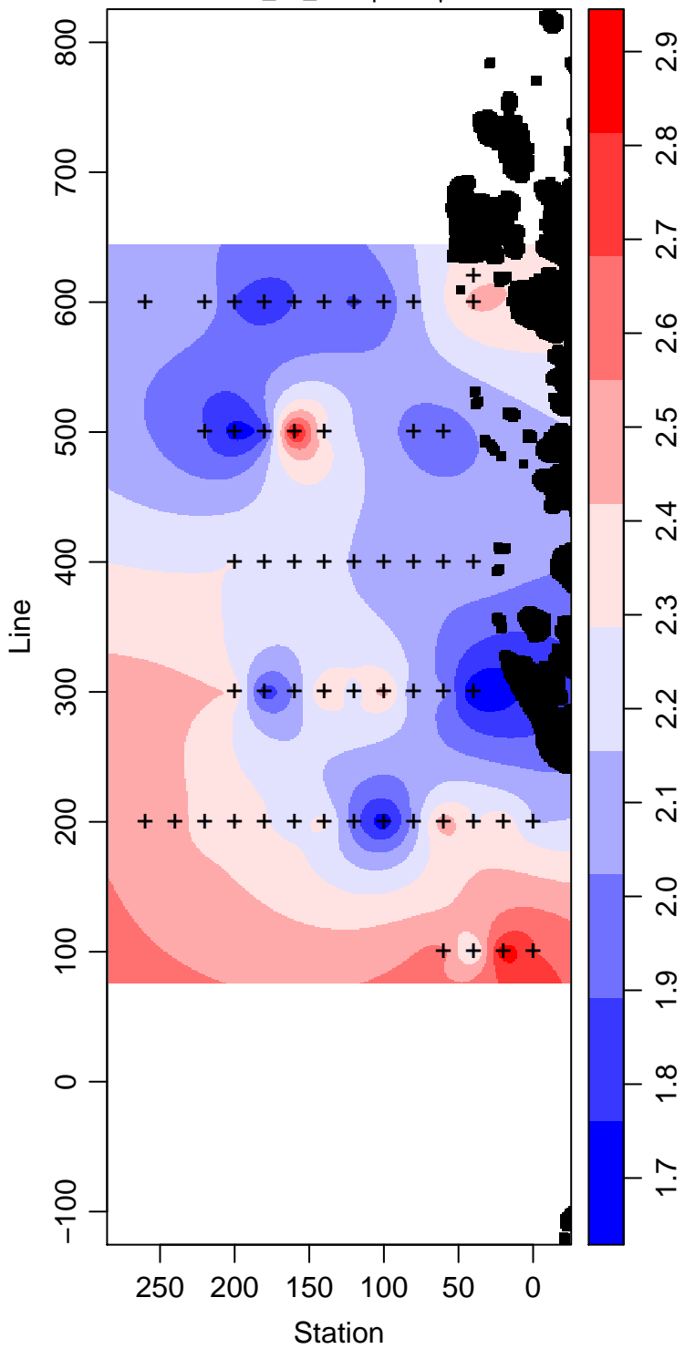
LMG07-01_65_Phosphate \mu\text{ mol L}^{-1}
