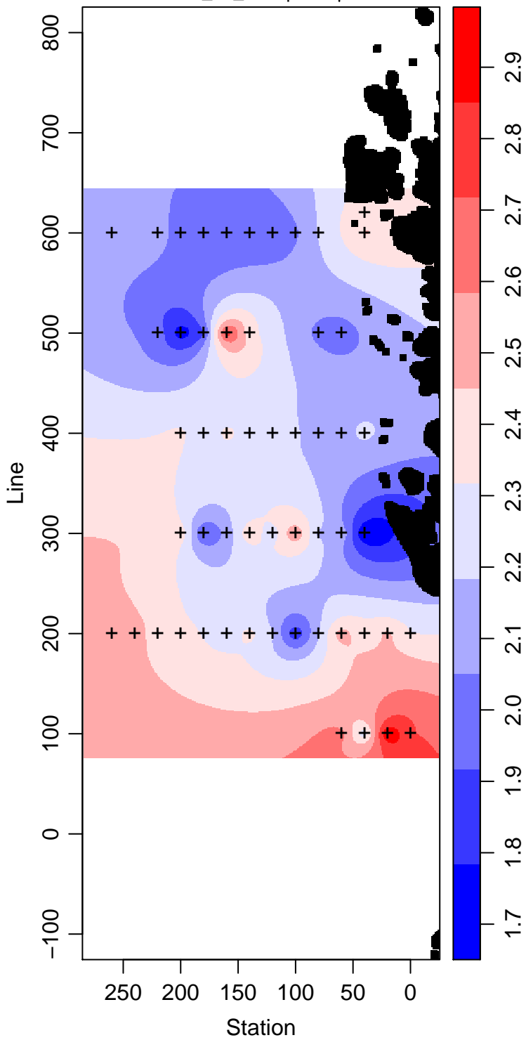
LMG07-01_70_Phosphate \mu\text{ mol L}^{-1}
