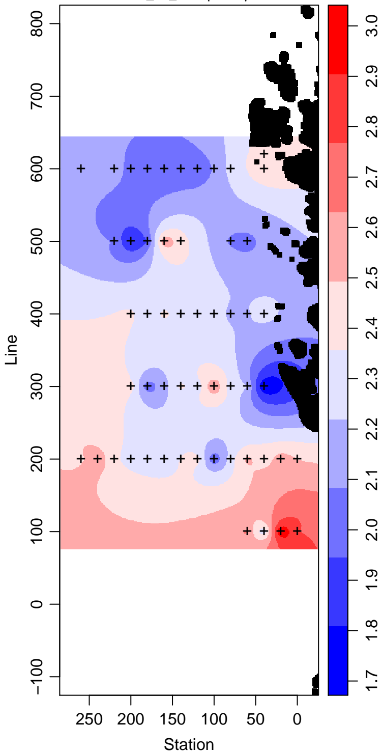
LMG07-01_75_Phosphate \mu\text{ mol L}^{-1}
