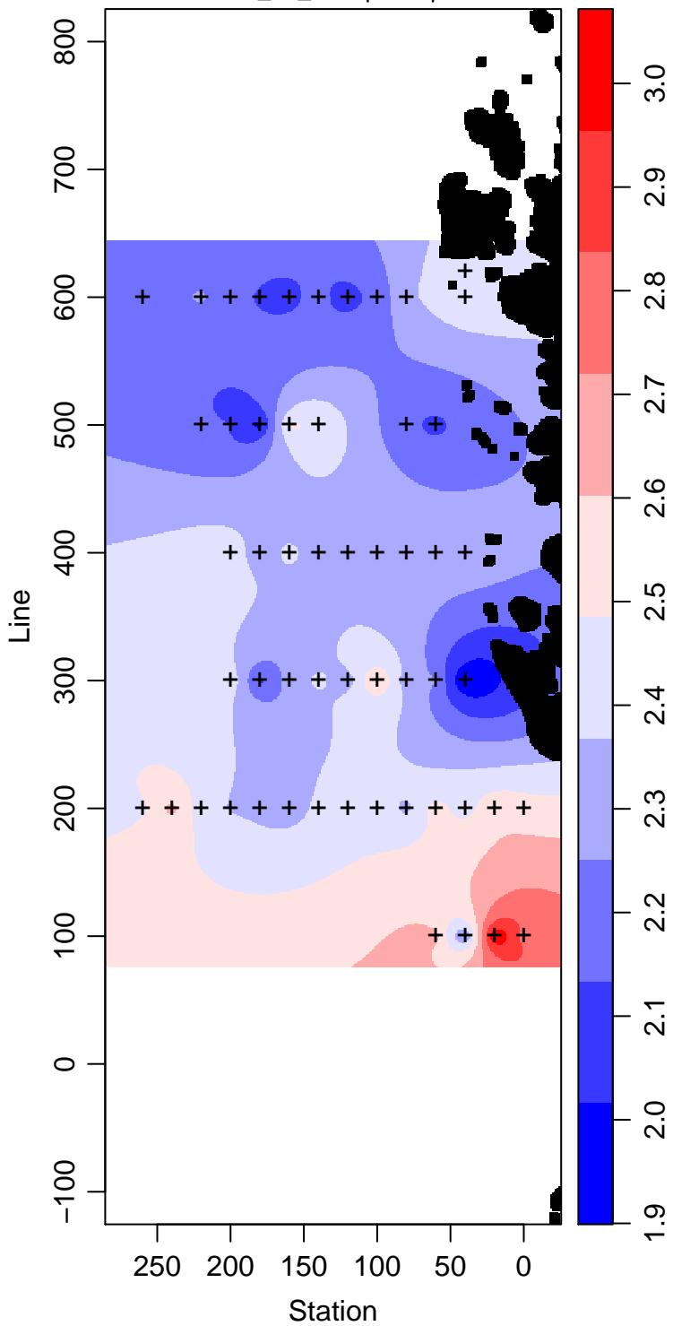
LMG07-01_85_Phosphate \mu\text{ mol L}^{-1}
