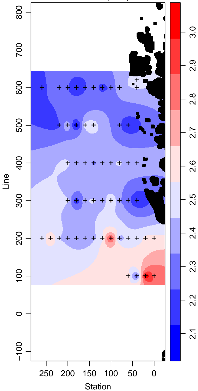
LMG07-01_95_Phosphate \mu\text{ mol L}^{-1}
