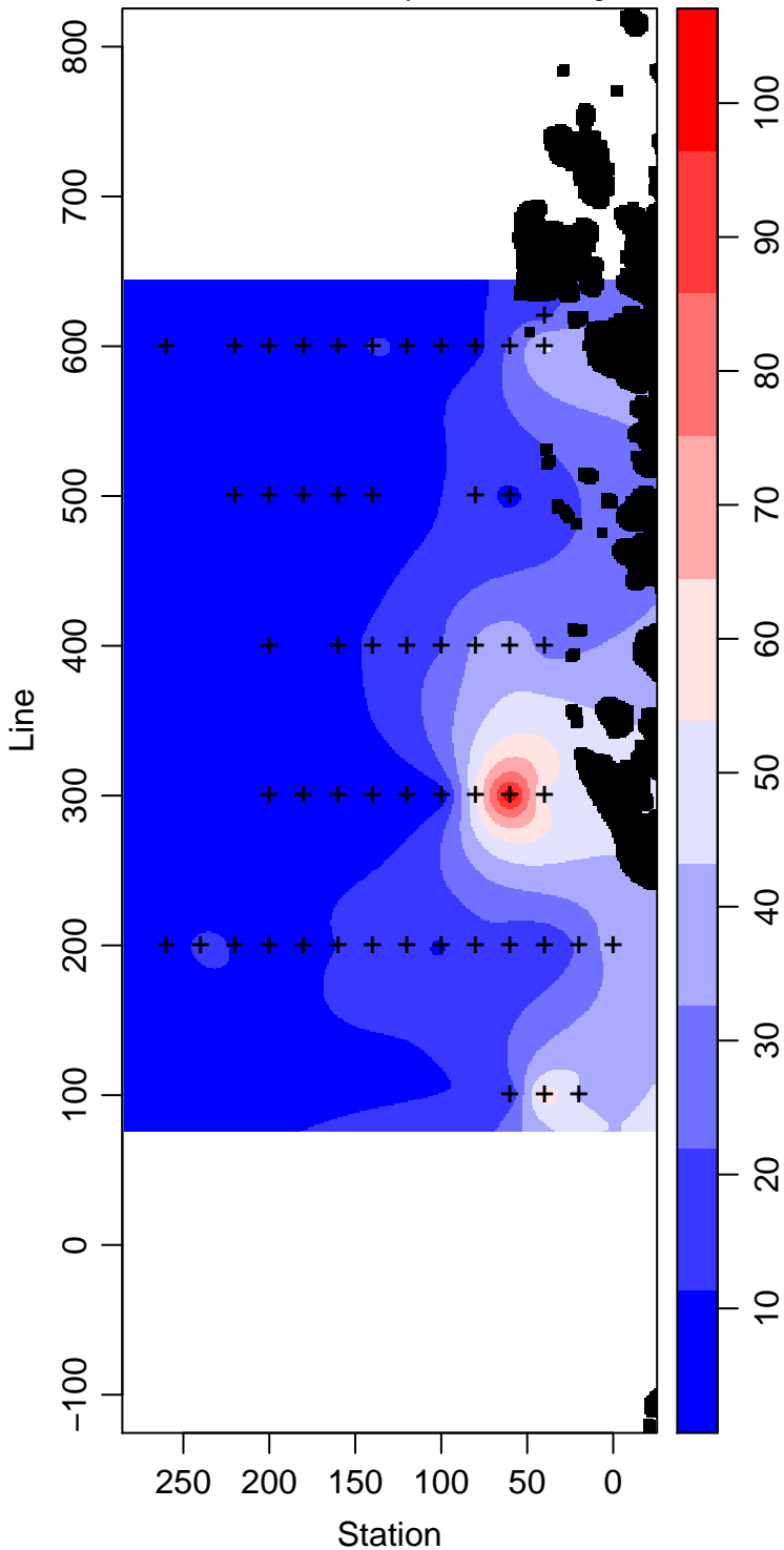
LMG07-01_15_Primary.Production mg m -3
