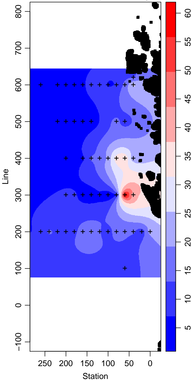
LMG07-01_20_Primary.Production mg m -3
