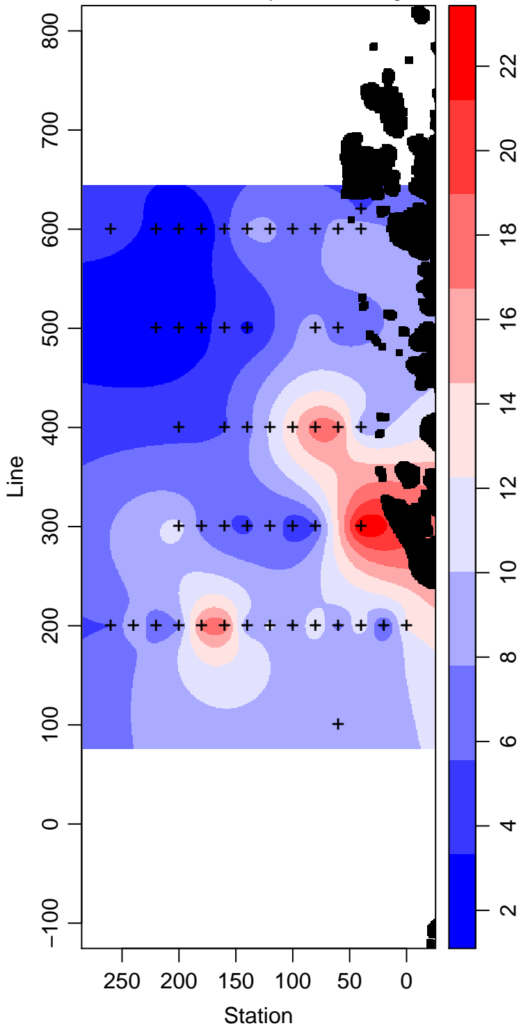
LMG07-01_30_Primary.Production mg m -3
