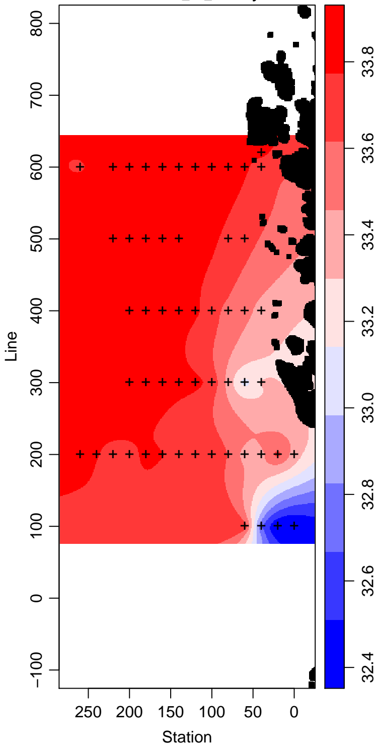
LMG07-01_15_Salinity
