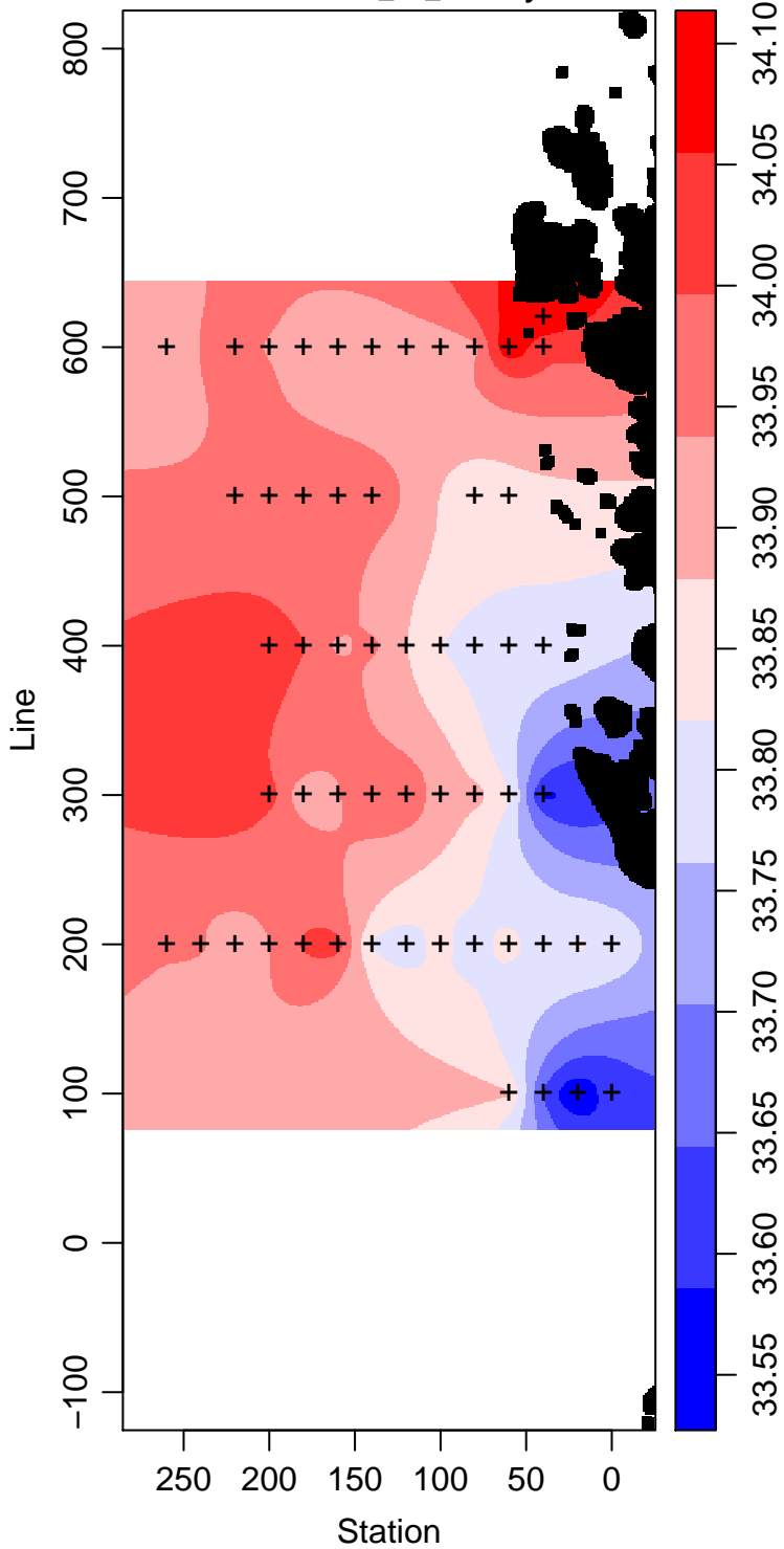
LMG07-01_50_Salinity
