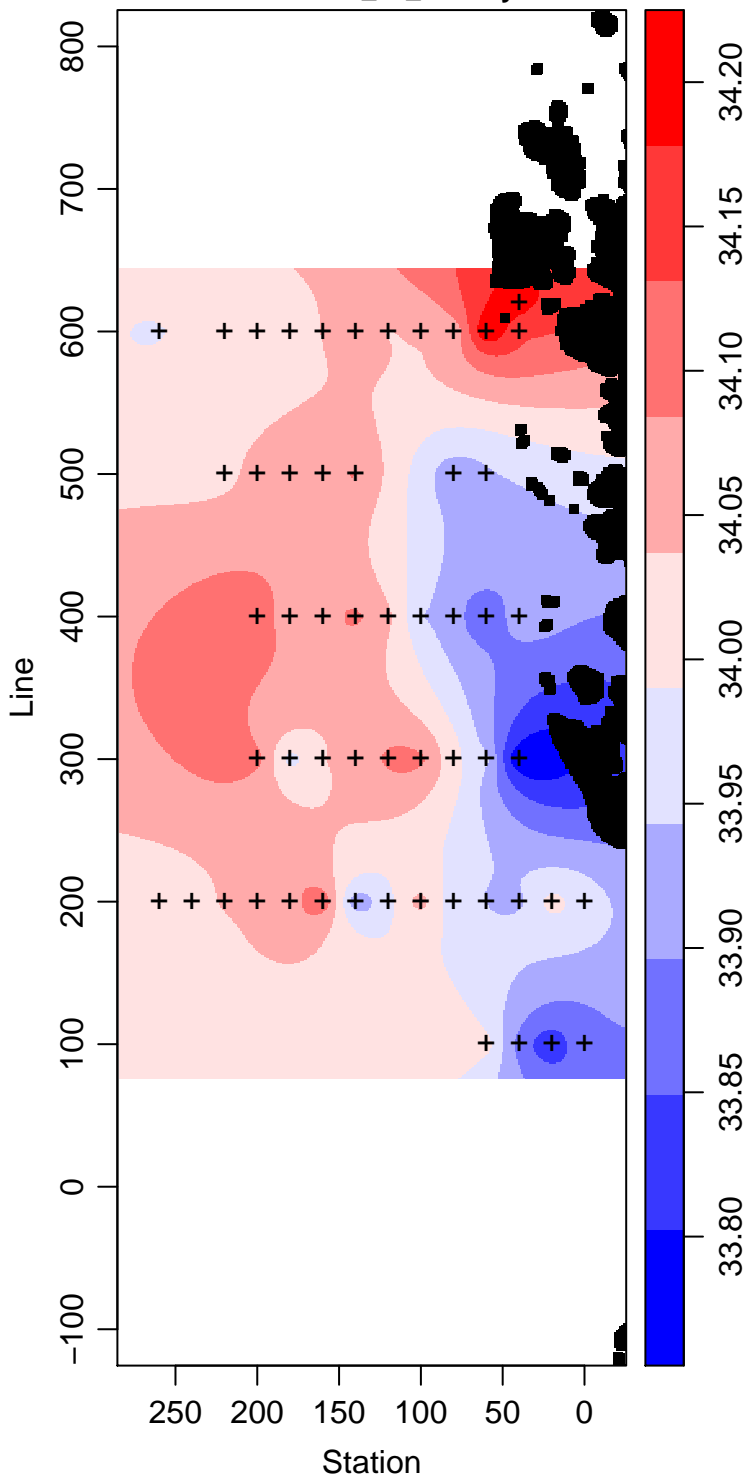
LMG07-01_70_Salinity
