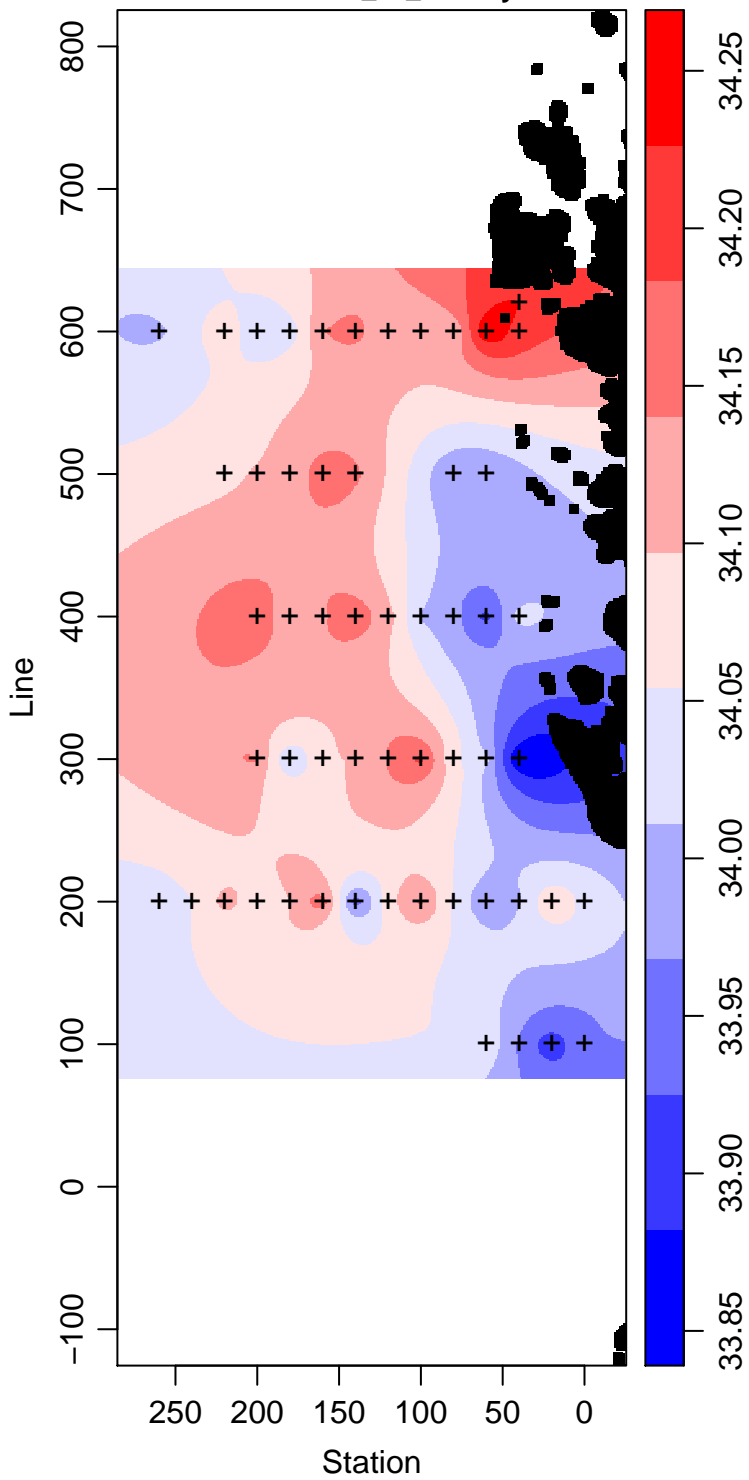
LMG07-01_80_Salinity
