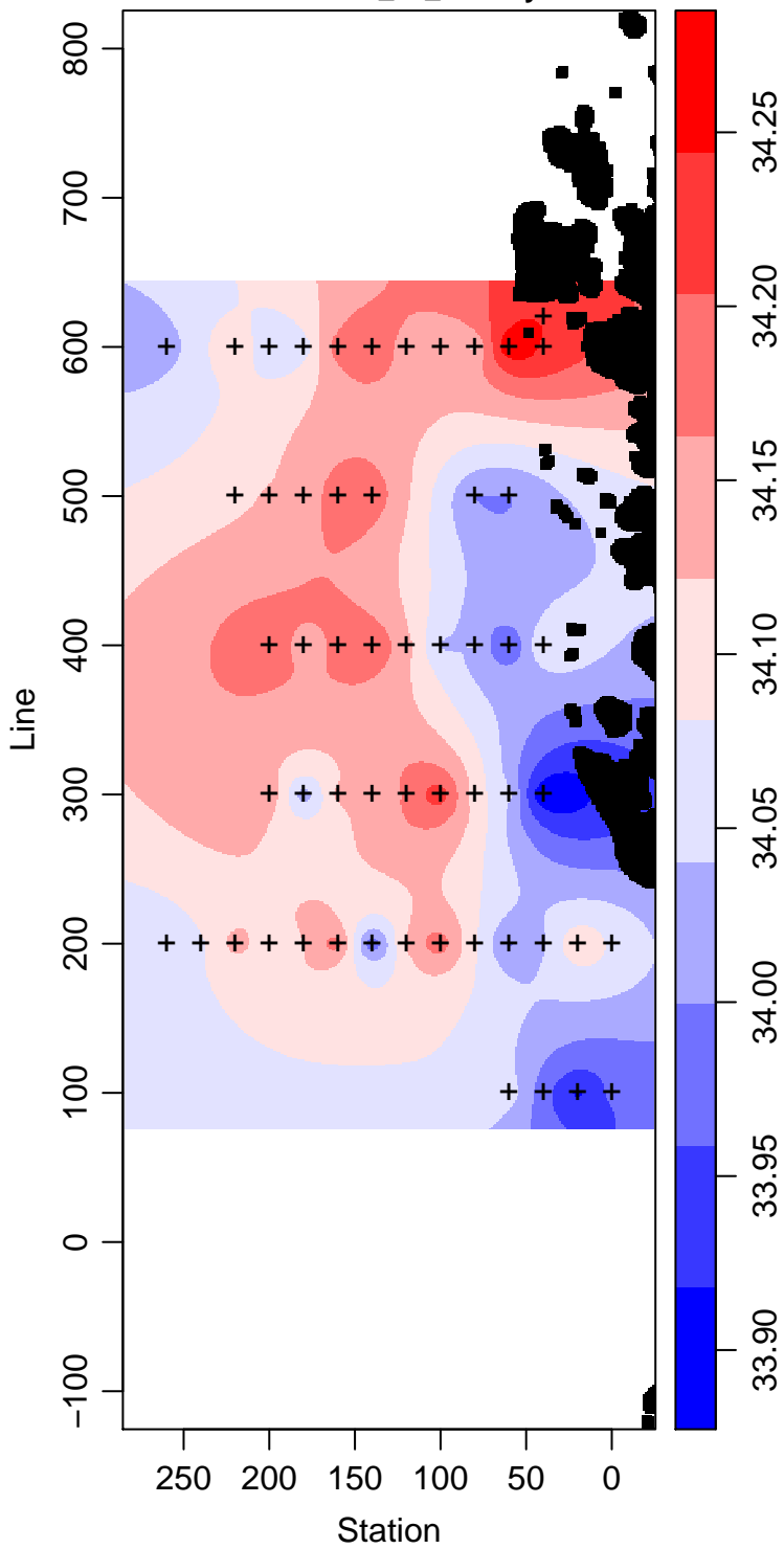
LMG07-01_85_Salinity
