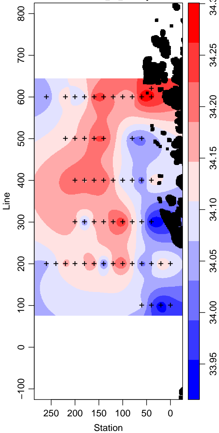
LMG07-01_90_Salinity
