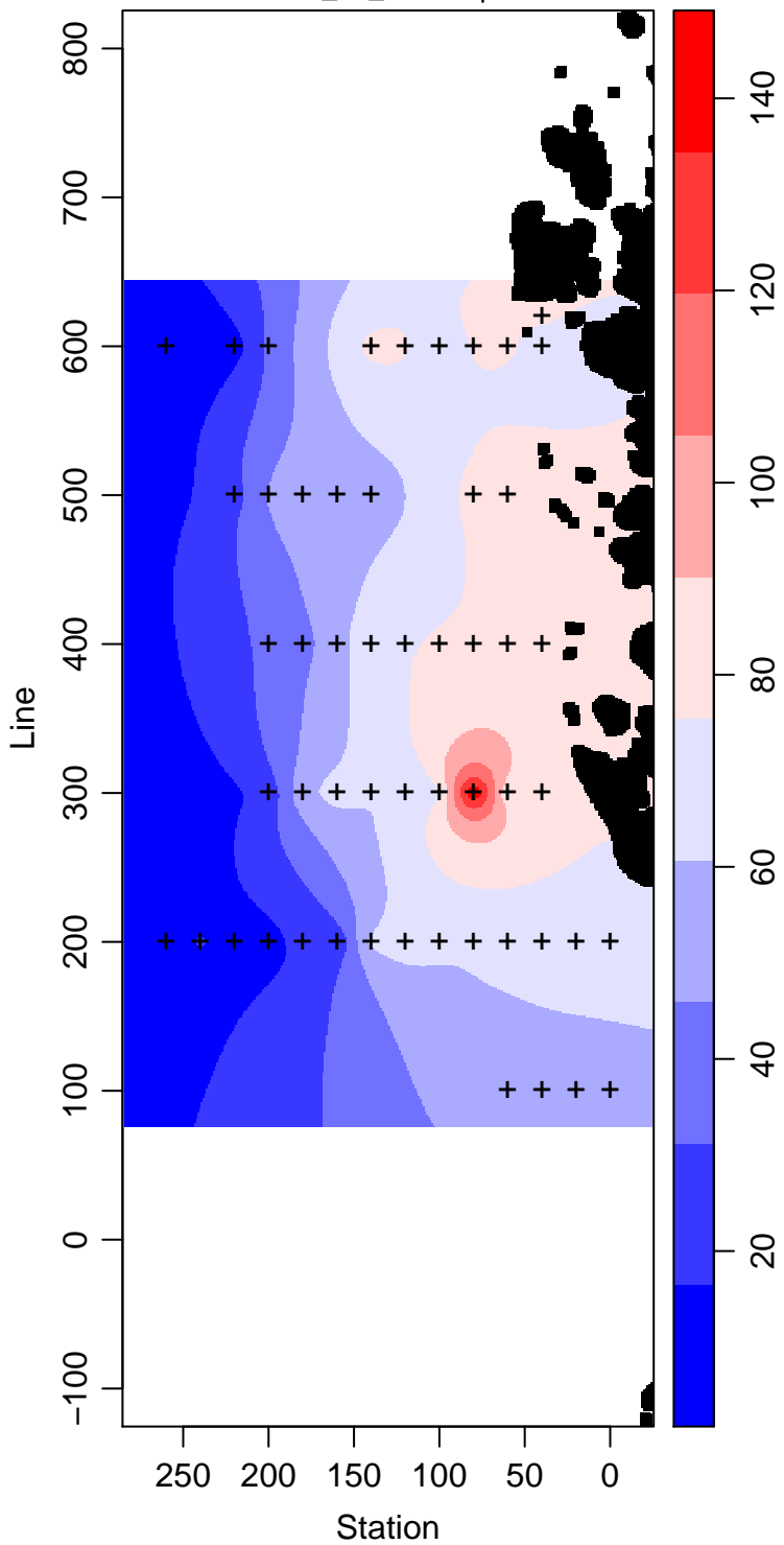
LMG07-01_10_Silicate \mu\text{ mol L}^{-1}
