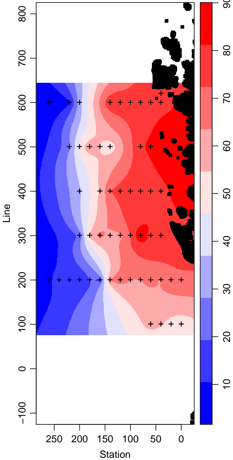
LMG07-01_1_Silicate \mu\text{ mol L}^{-1}
