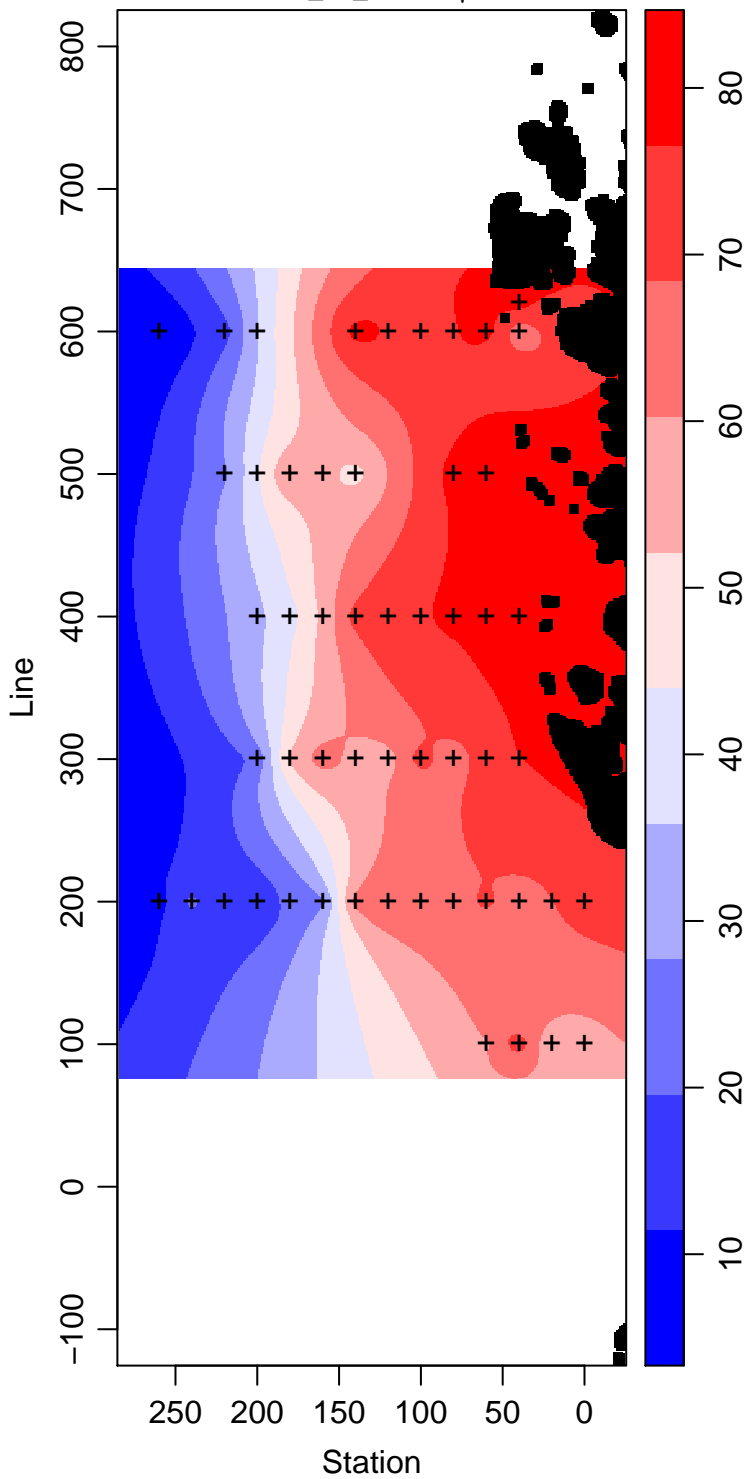
LMG07-01_20_Silicate \mu\text{ mol L}^{-1}
