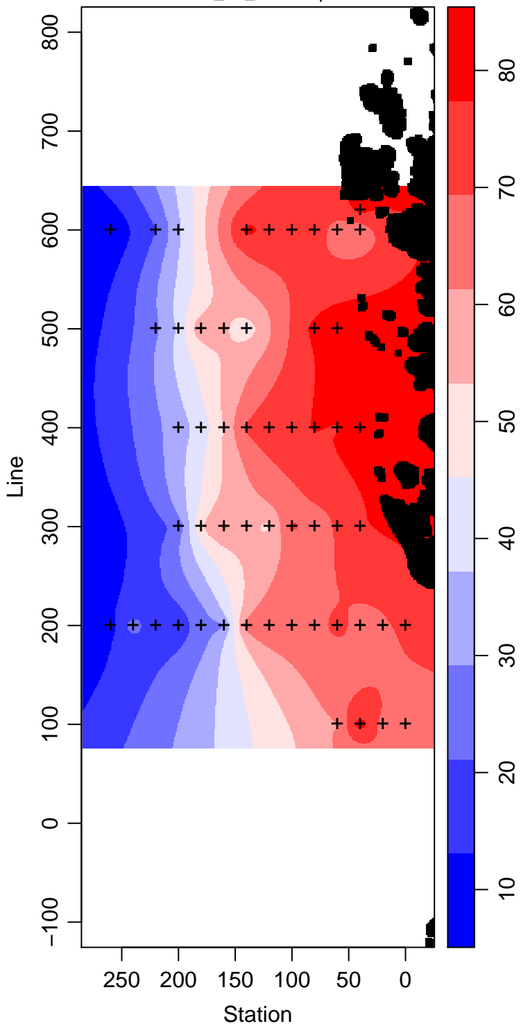
LMG07-01_25_Silicate \mu\text{ mol L}^{-1}
