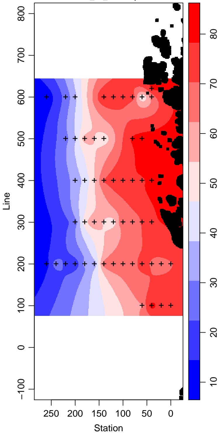
LMG07-01_30_Silicate \mu\text{ mol L}^{-1}
