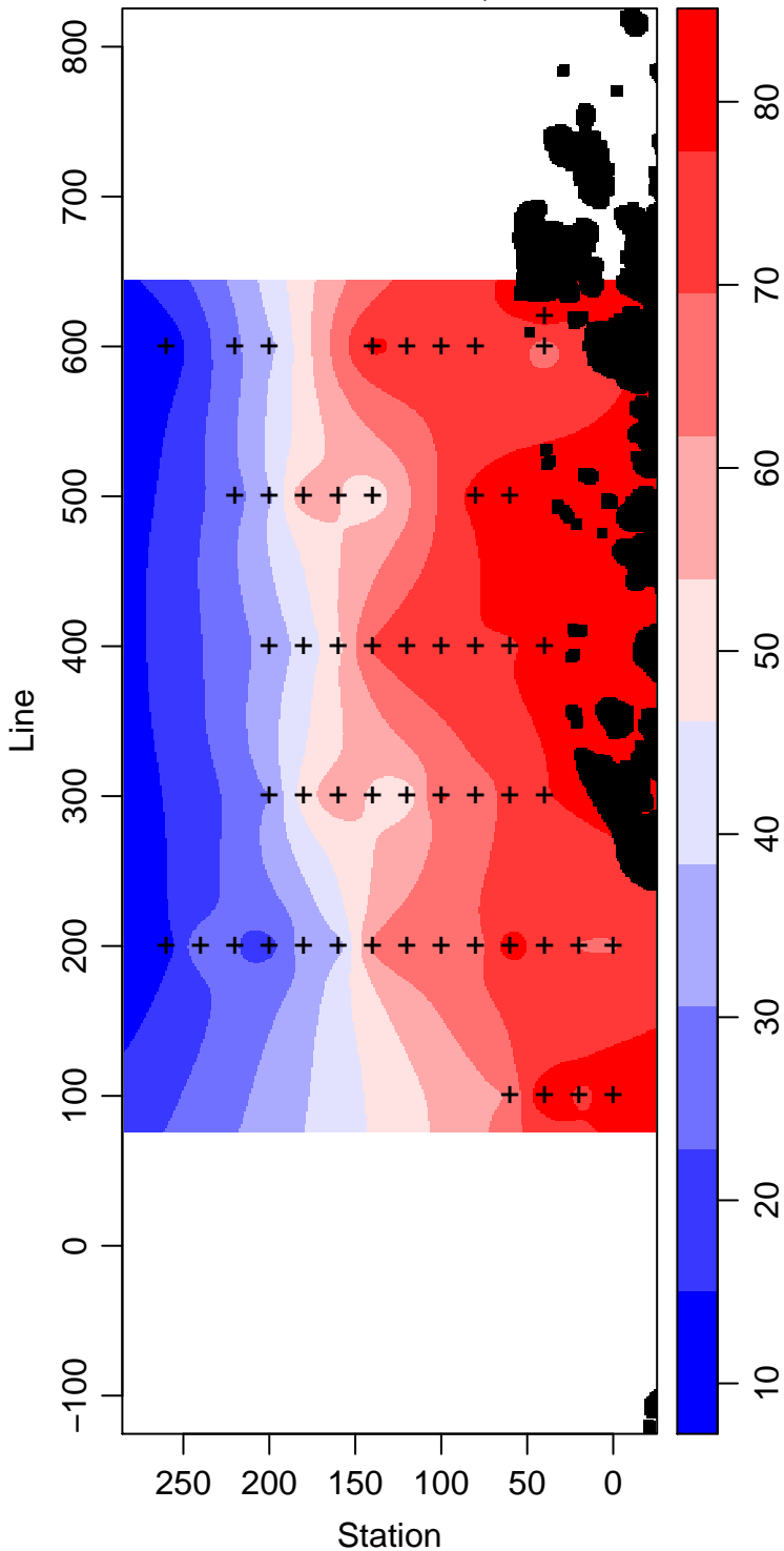
LMG07-01_35_Silicate \mu\text{ mol L}^{-1}
