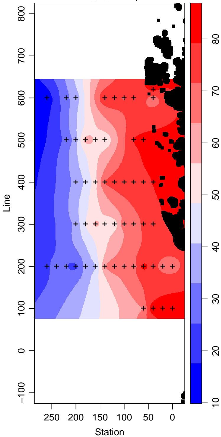
LMG07-01_40_Silicate \mu\text{ mol L}^{-1}
