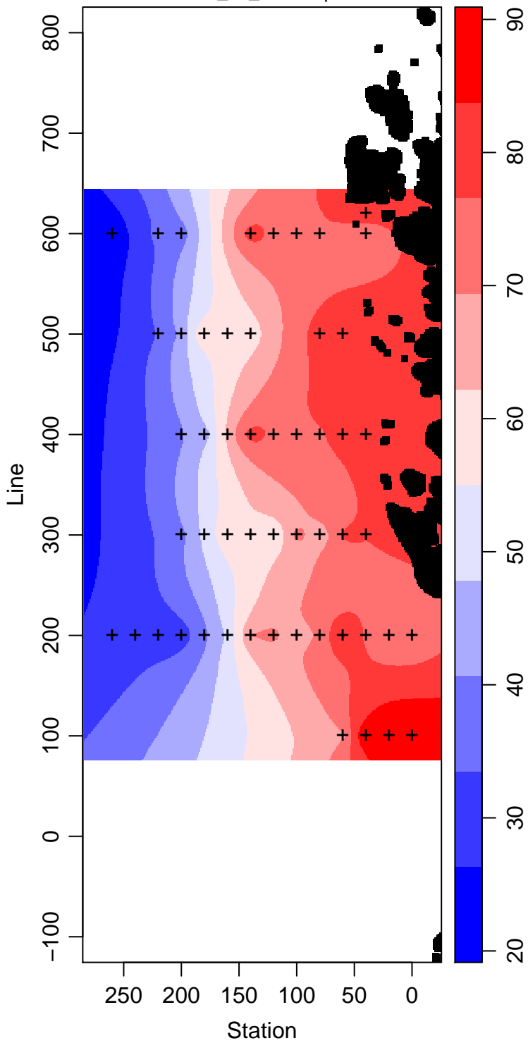
LMG07-01_50_Silicate \mu\text{ mol L}^{-1}
