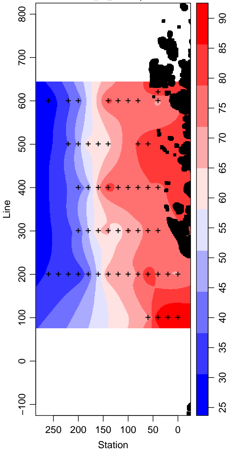
LMG07-01_55_Silicate \mu\text{ mol L}^{-1}
