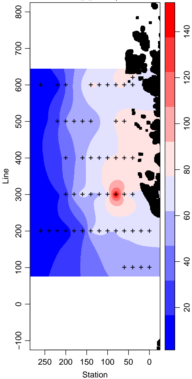
LMG07-01_5_Silicate \mu\text{ mol L}^{-1}
