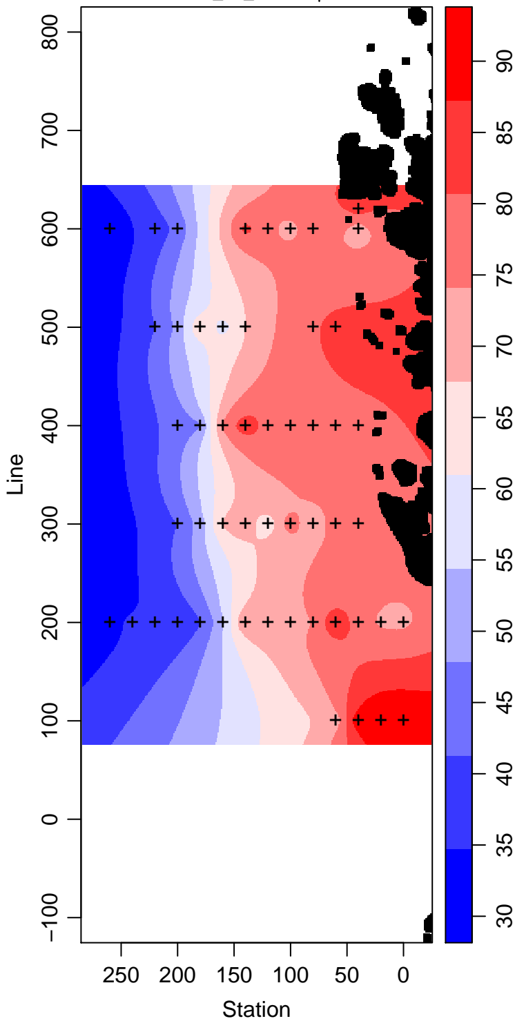
LMG07-01_60_Silicate \mu\text{ mol L}^{-1}
