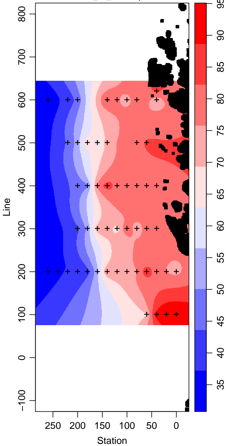
LMG07-01_65_Silicate \mu\text{ mol L}^{-1}
