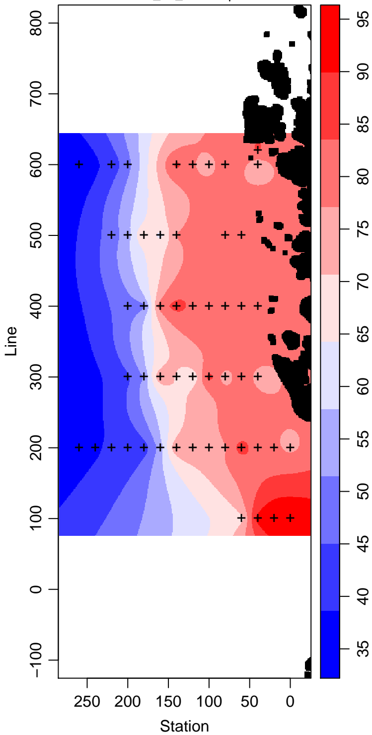
LMG07-01_70_Silicate \mu\text{ mol L}^{-1}
