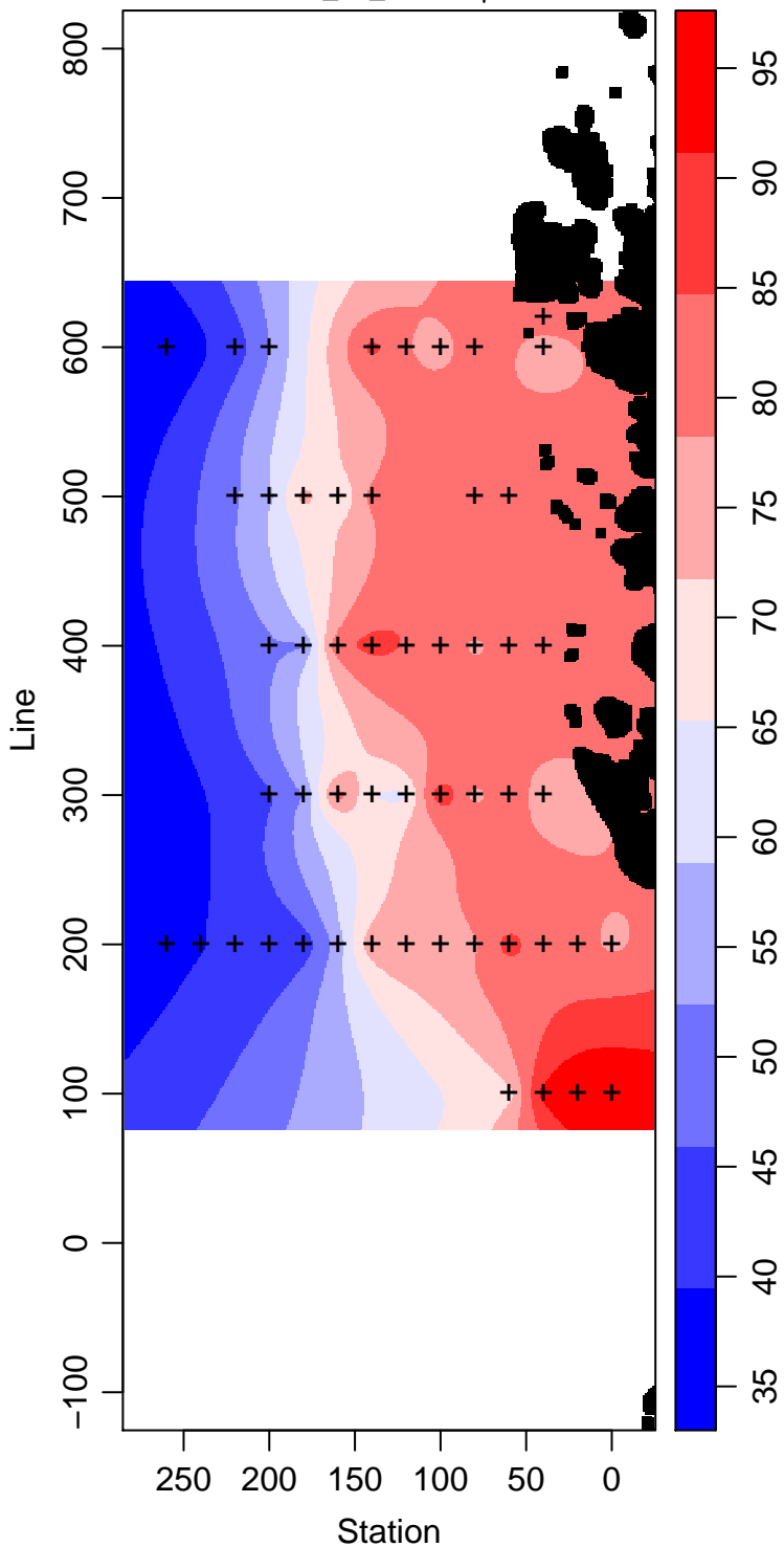
LMG07-01_75_Silicate \mu\text{ mol L}^{-1}
