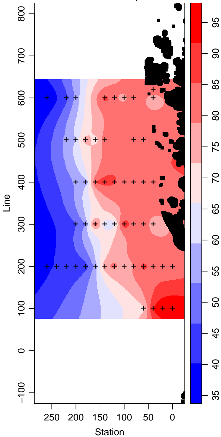
LMG07-01_80_Silicate \mu\text{ mol L}^{-1}
