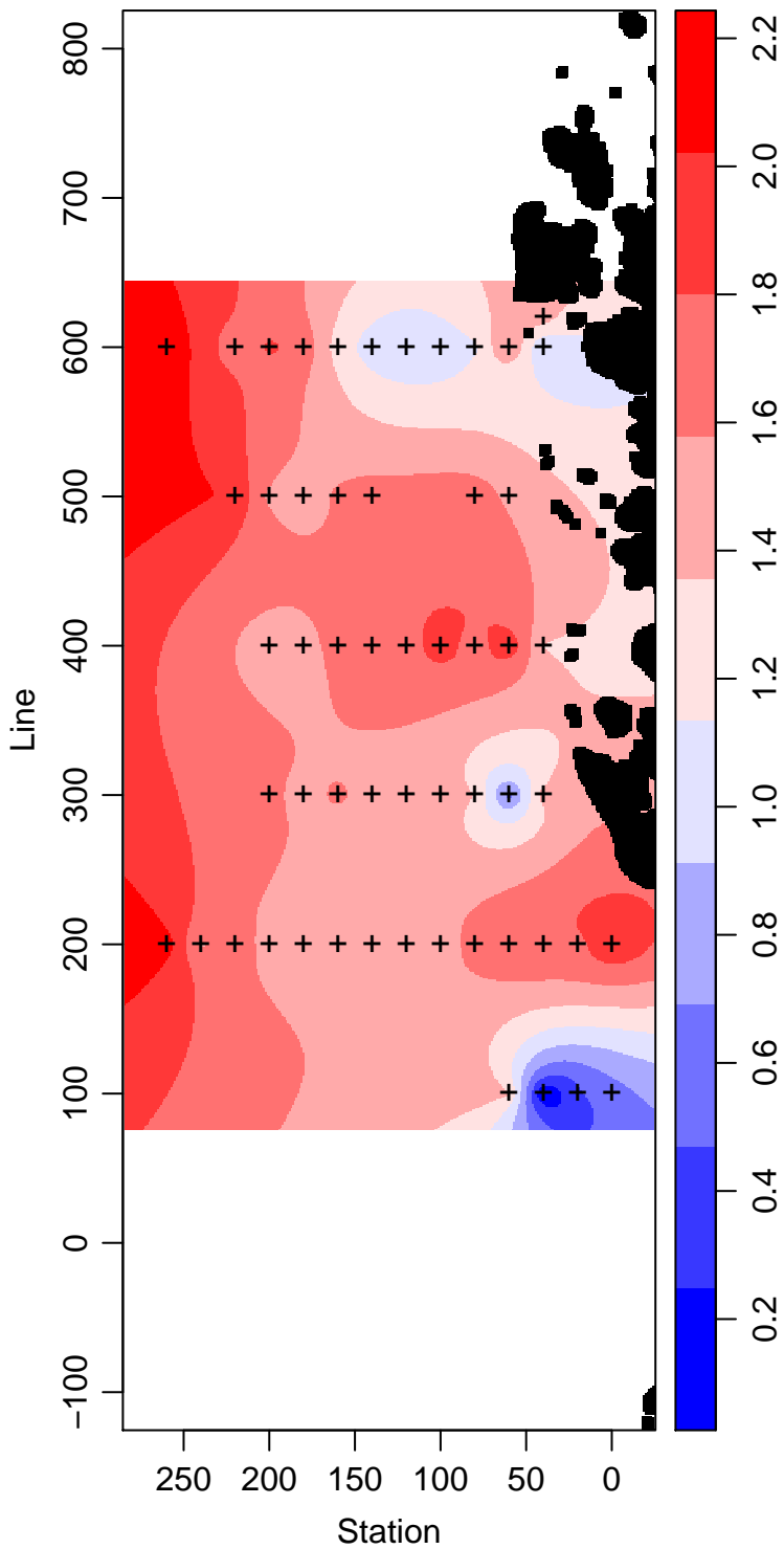
LMG07-01_15_Temperature ° Celsius
