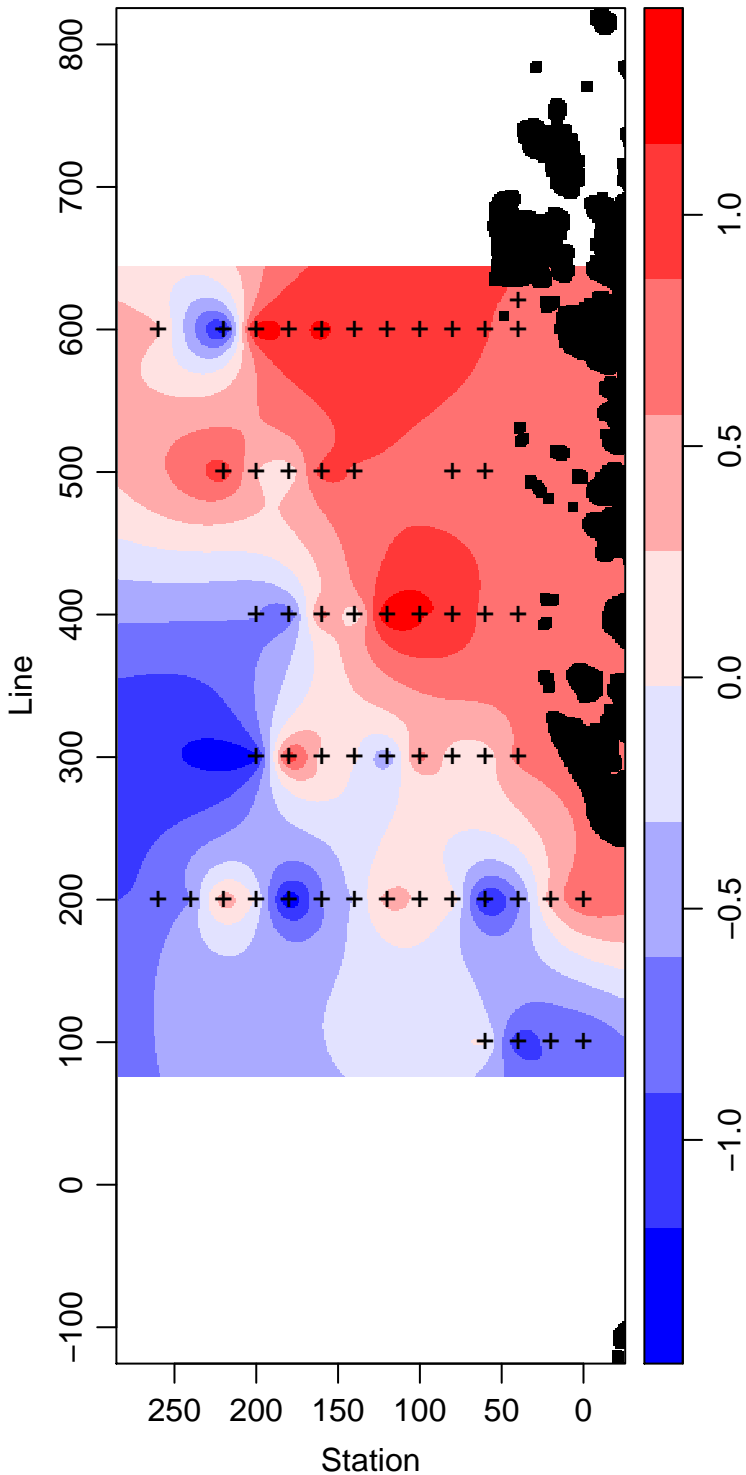
LMG07-01_45_Temperature ° Celsius
