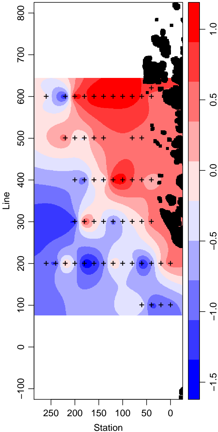
LMG07-01_50_Temperature ° Celsius
