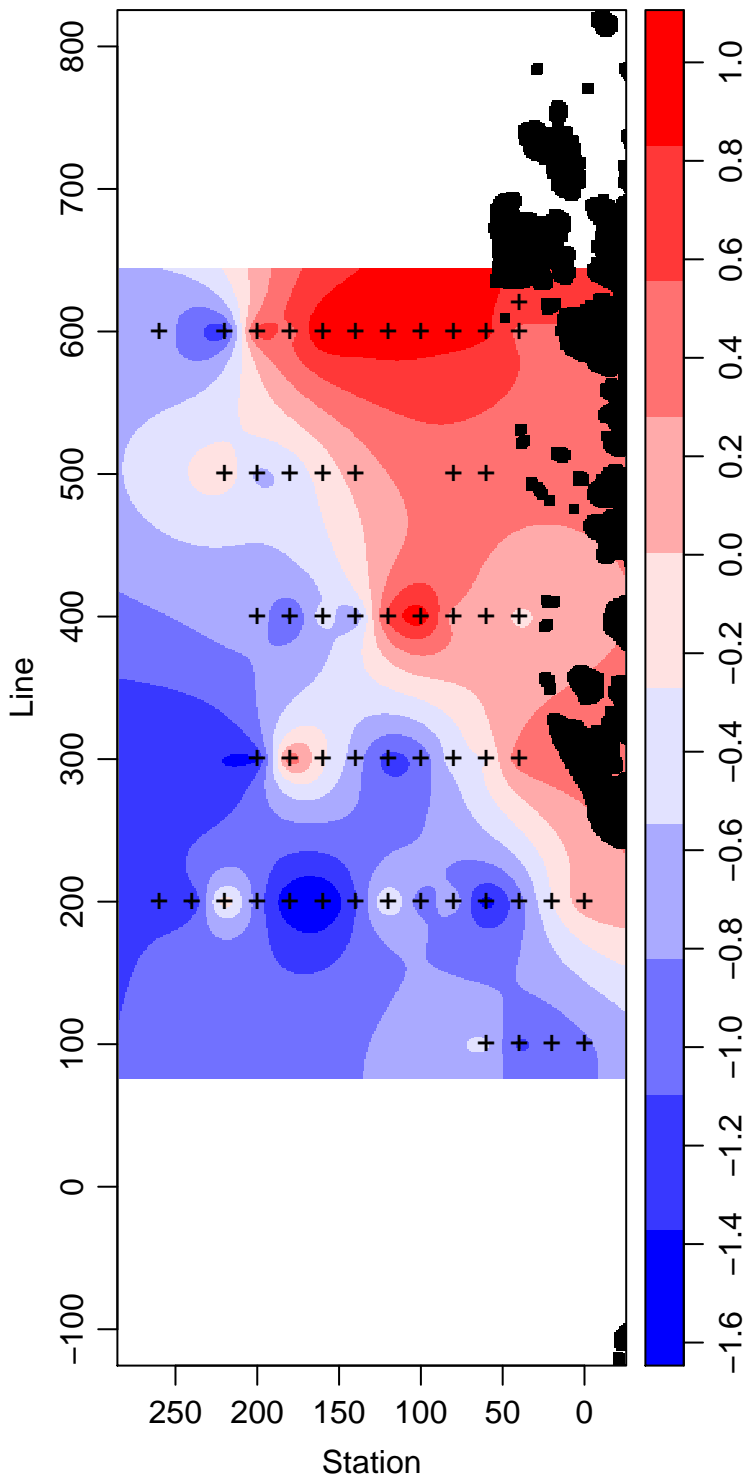
LMG07-01_55_Temperature ° Celsius
