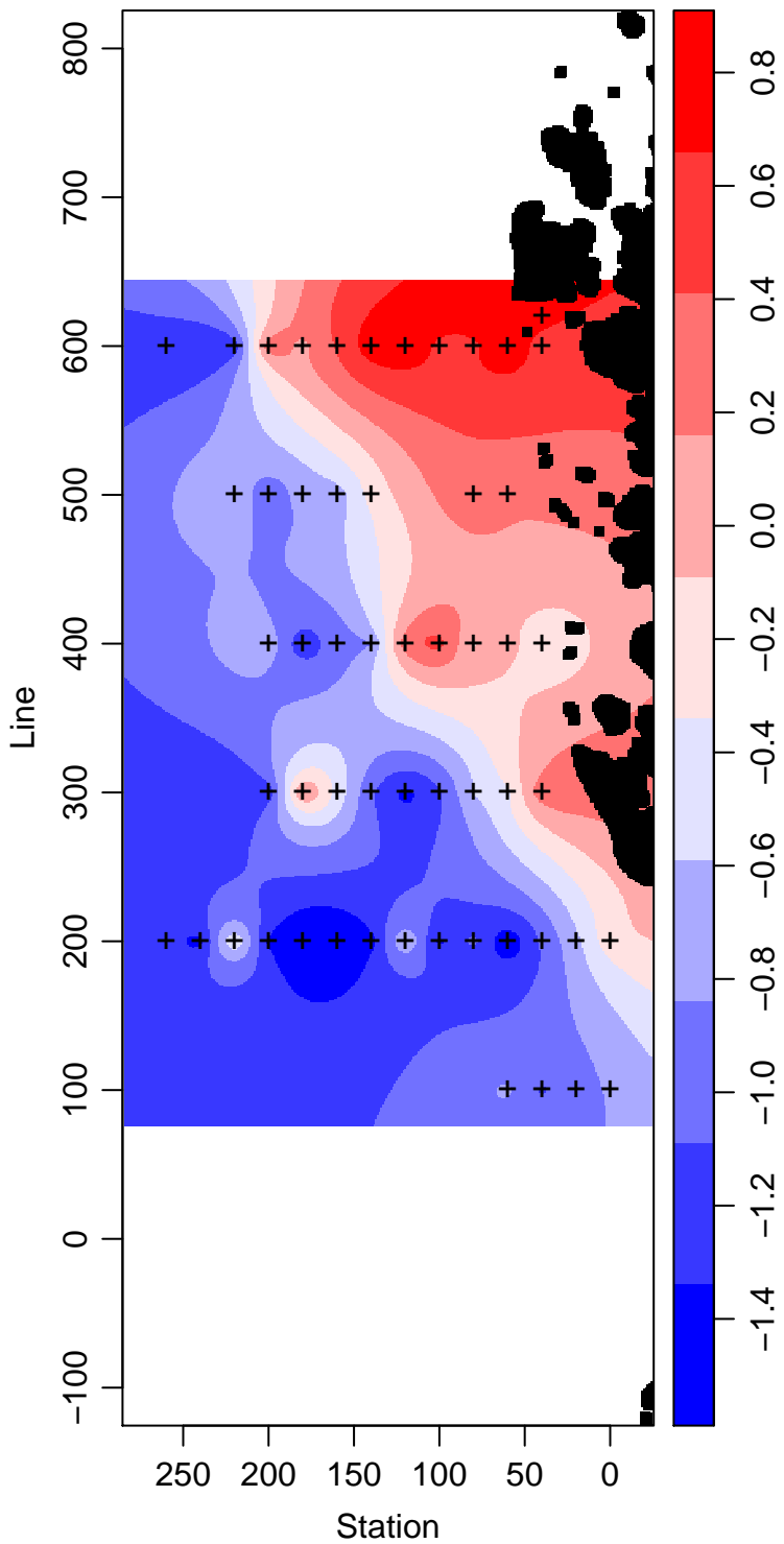
LMG07-01_60_Temperature ° Celsius
