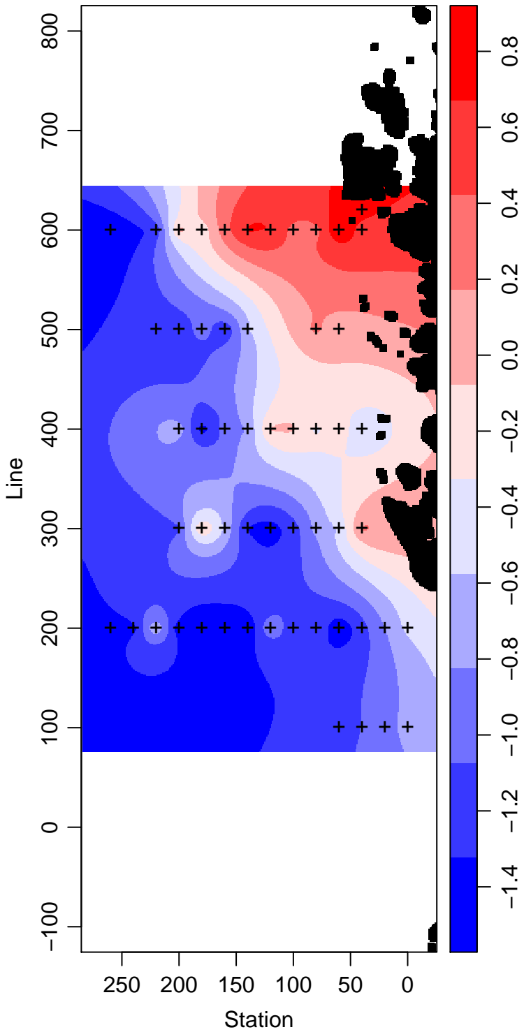
LMG07-01_65_Temperature ° Celsius
