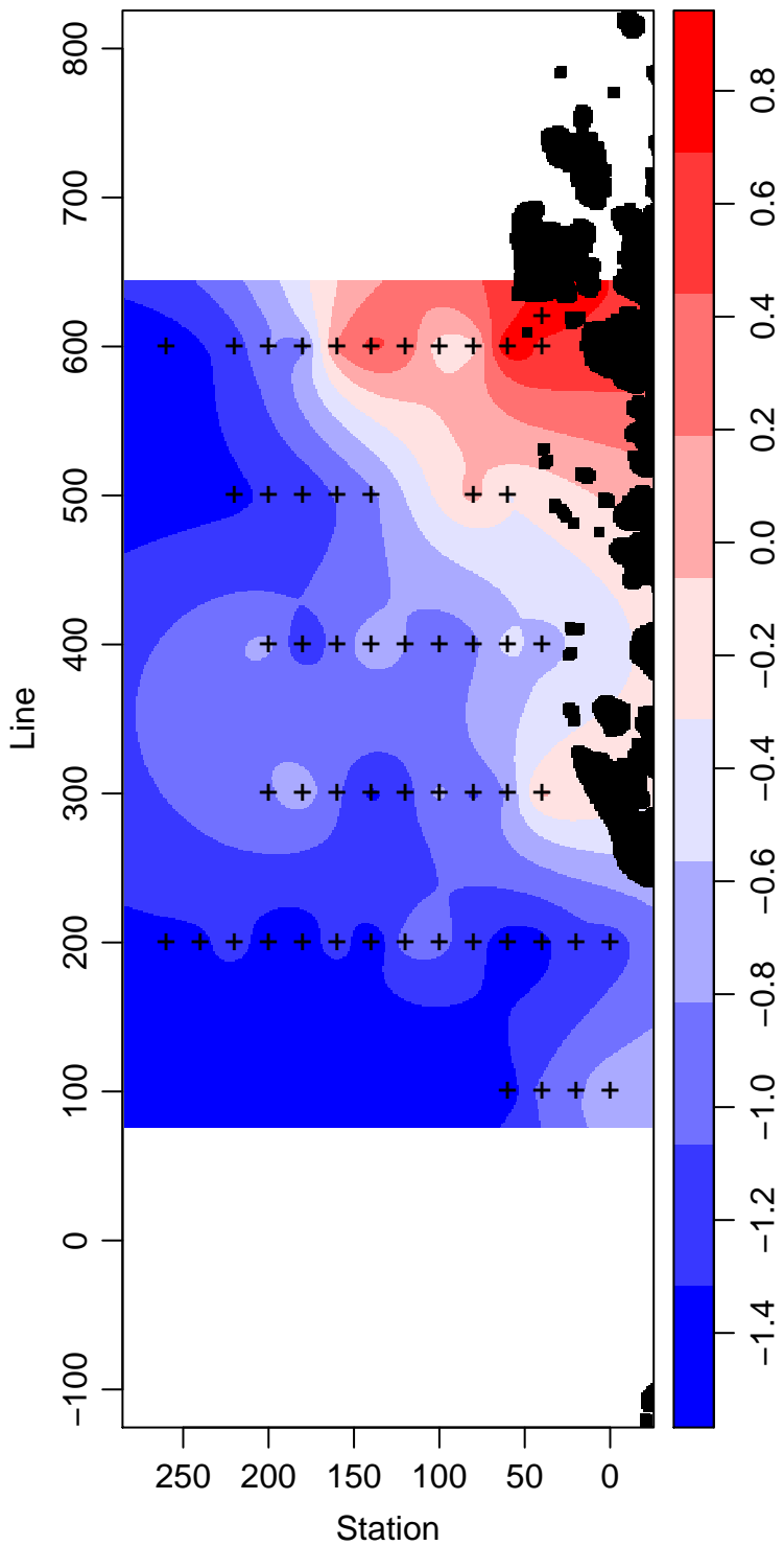
LMG07-01_75_Temperature ° Celsius
