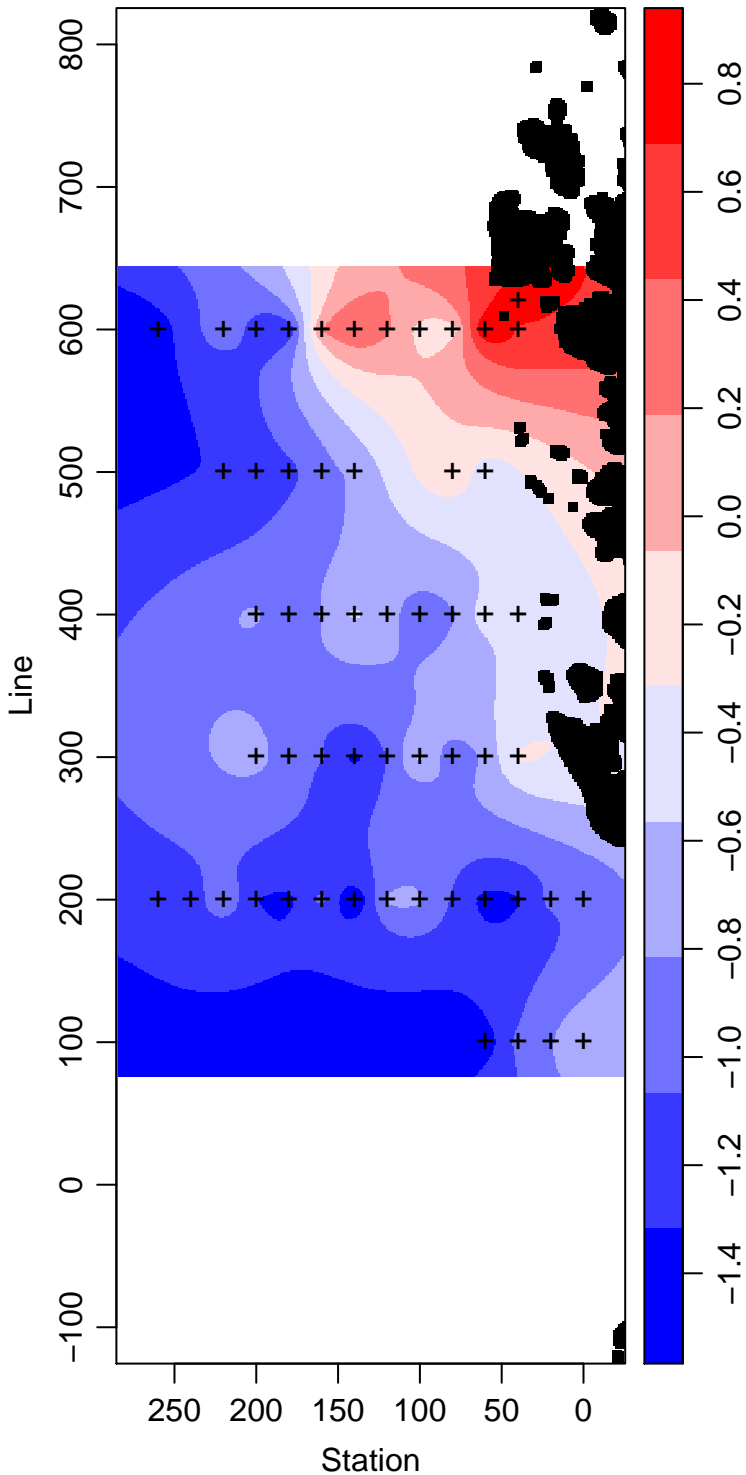
LMG07-01_80_Temperature ° Celsius
