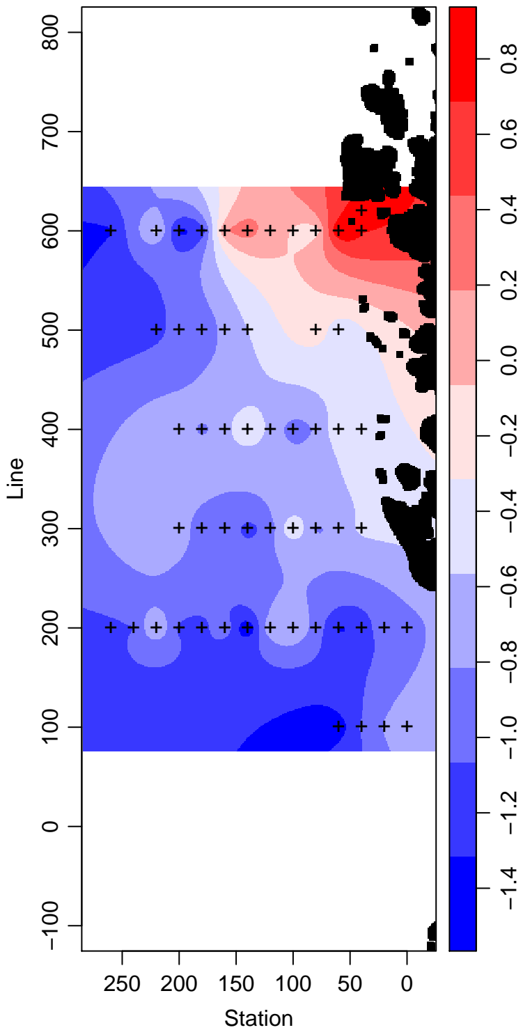
LMG07-01_85_Temperature ° Celsius
