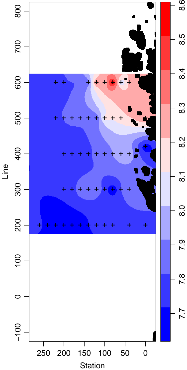
LMG08-01_10_Dissolved.Oxygen ml L -1
