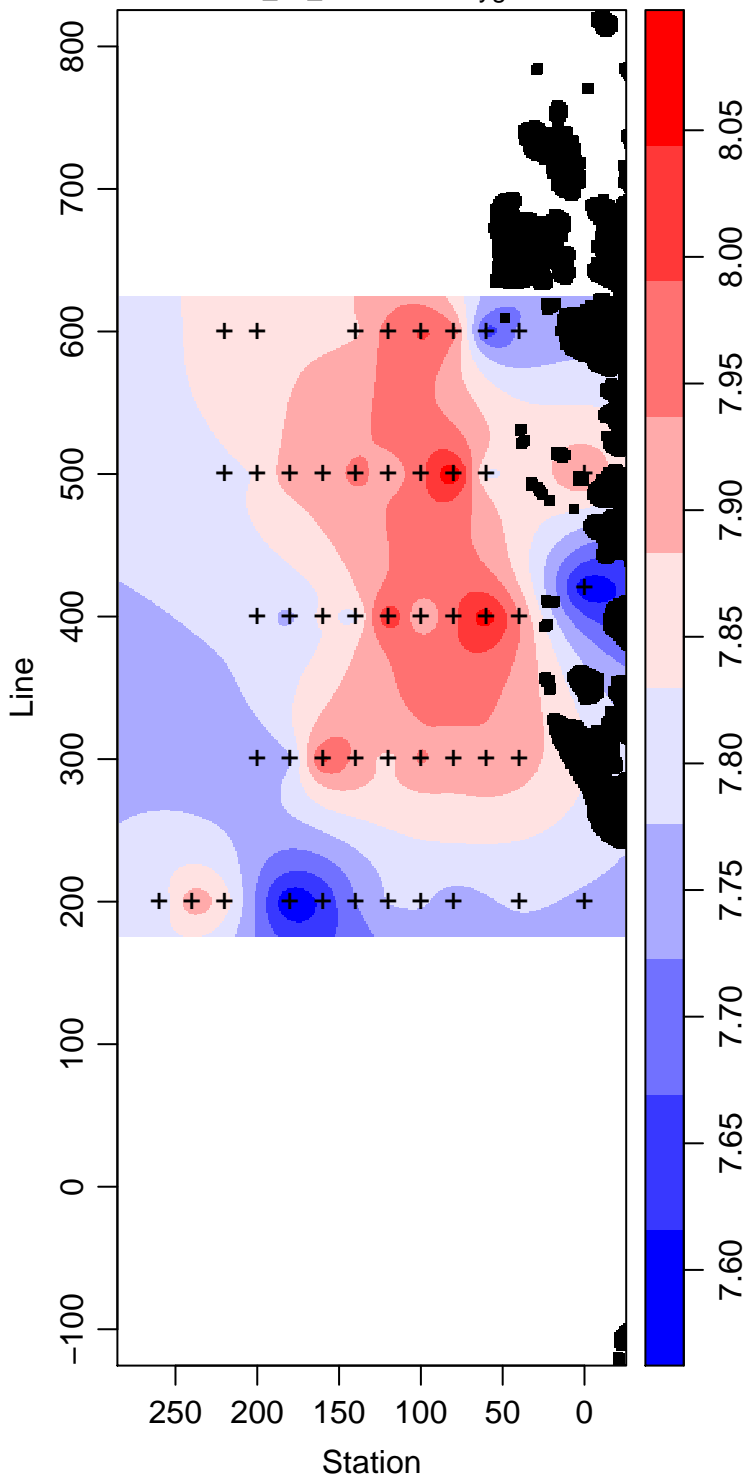
LMG08-01_30_Dissolved.Oxygen ml L -1
