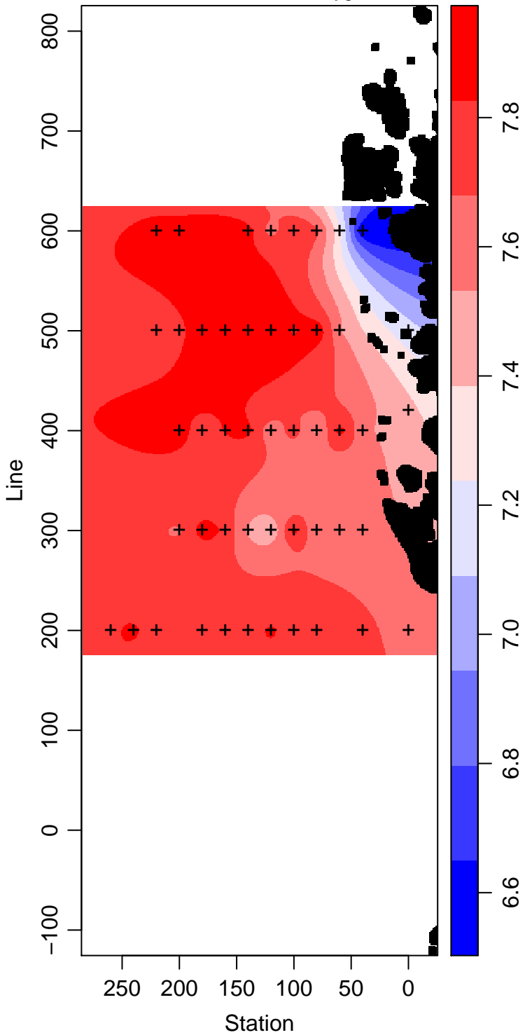
LMG08-01_55_Dissolved.Oxygen ml L -1
